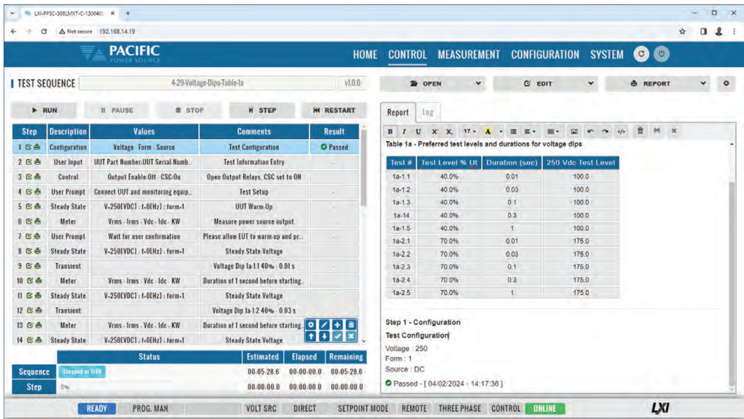
Figure 15: IEC 61000-4-29 Test Execution Control Screen
