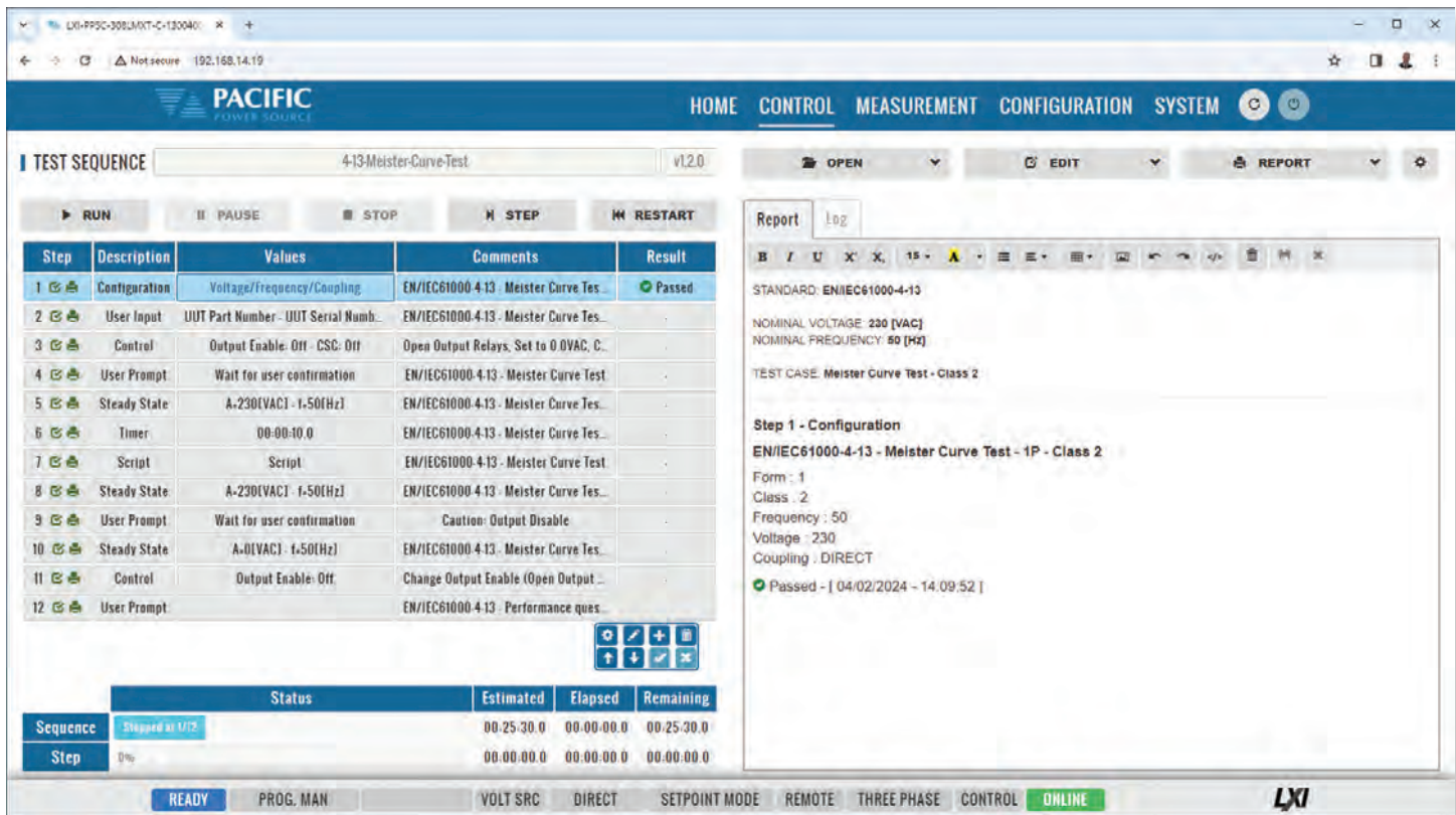
Figure 8: IEC 61000-4-13 Test Execution Control Screen
