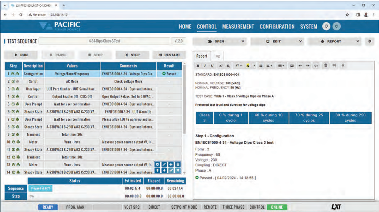
Figure 18: IEC 61000-4-34 Test Execution Control Screen
