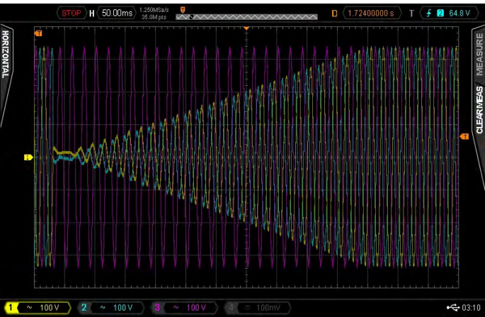
Figure 19: IEC 61000-4-34 Three Phase Voltage Variation Test
